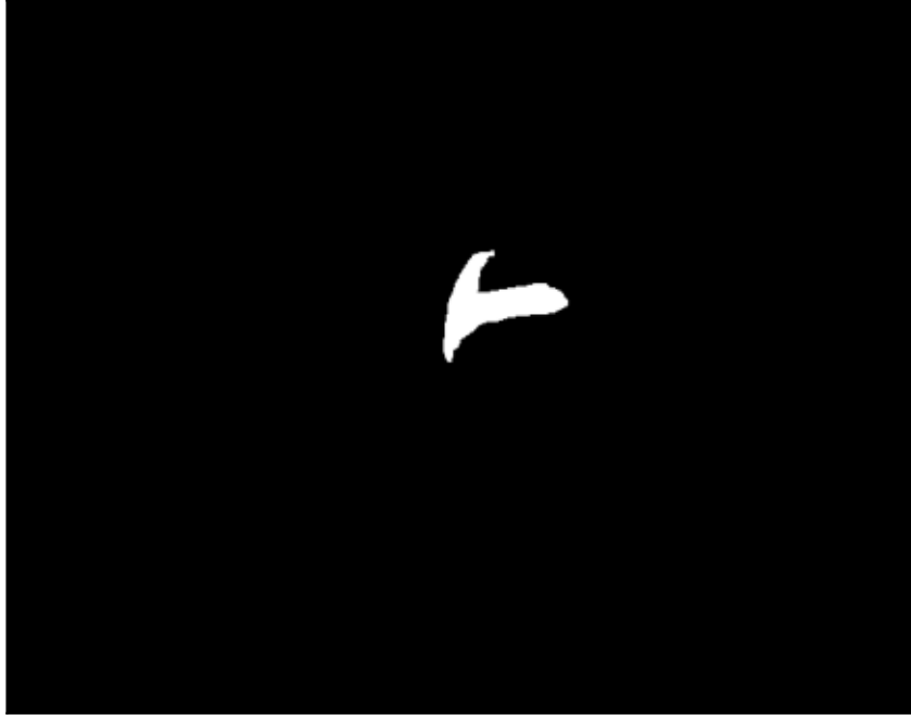
Segmentation Mask
